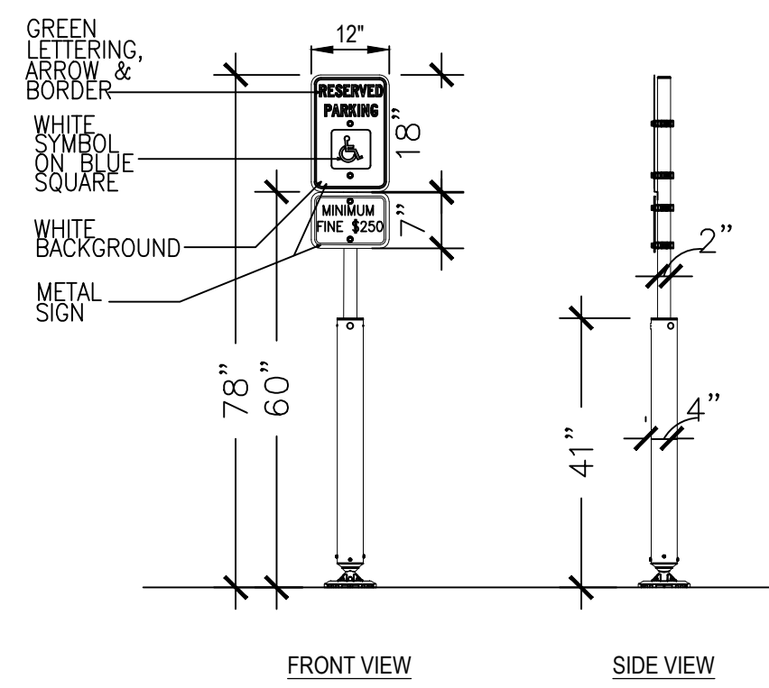
H/C DETAIL
